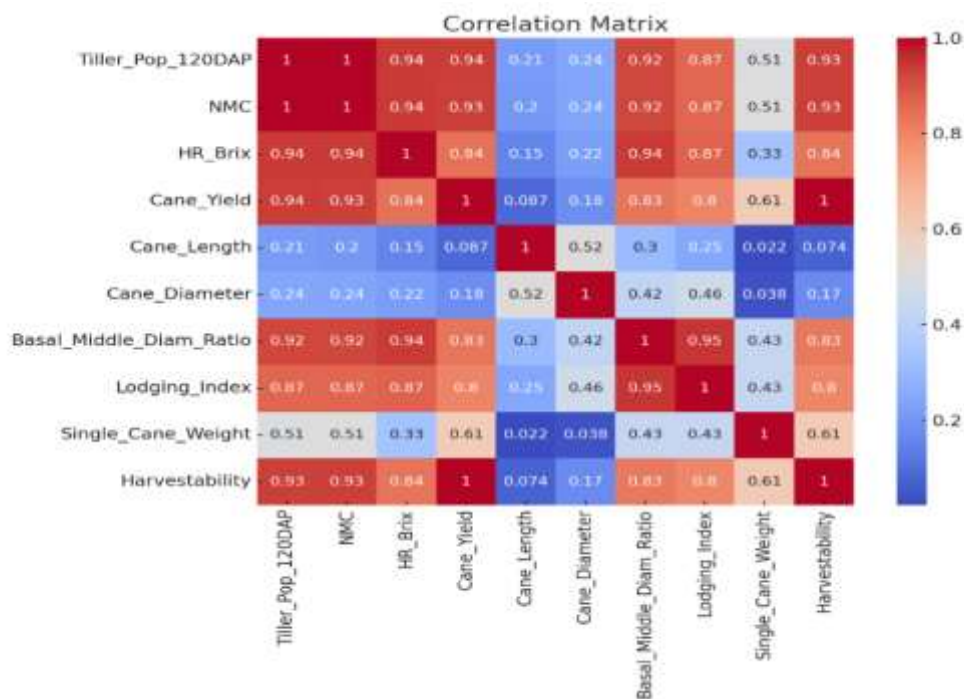
Fig. 1. Heat map of correlation matrix and Graphical representation of Actual and predicted harvestability with mechanical harvesting amicable traits.
